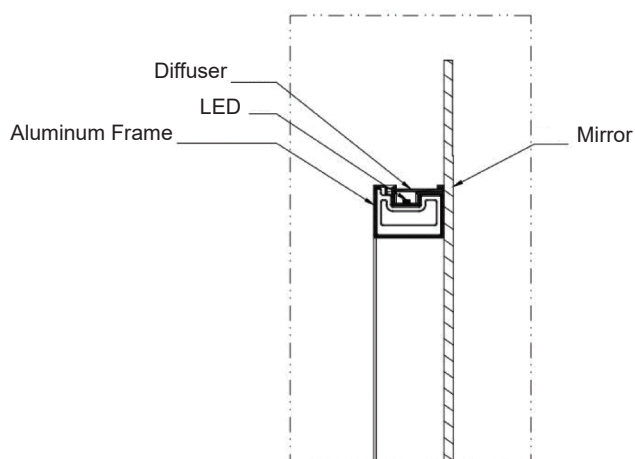
LED strip backlit construction from side view
