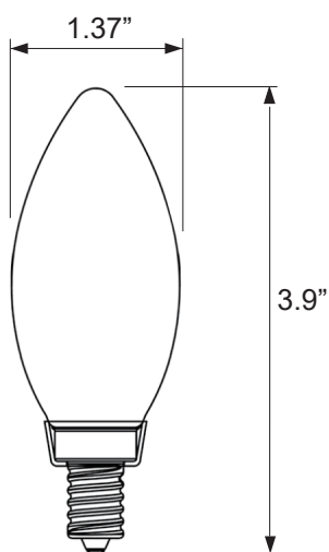
C35 Filament Bulb
